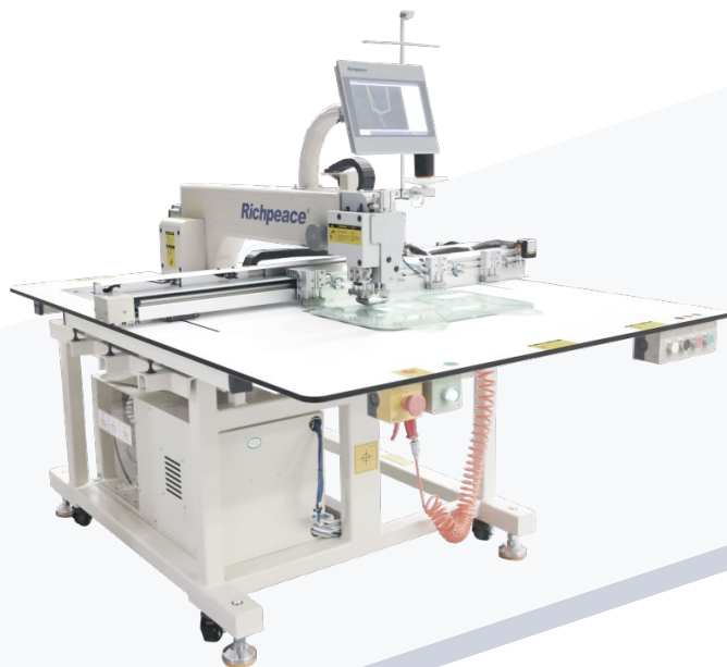
Model: RPAS-LM-C-1-1200x800-A-IS1-VR1-1P220 Work Area: 1200mmx800mm (XxY) Installation Size: 2400mmx2400mmx1500mm (LxWxH)
