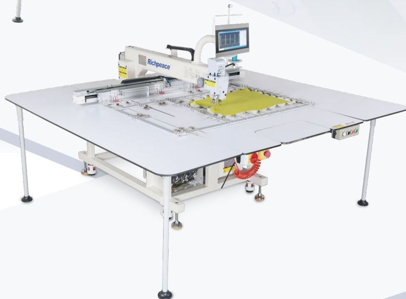
Model: RPAS-LM-C-1-1200x800-A-IS1-VR1-1P220 Work Area: 1200mmx800mm (XxY) Installation Size: 2400mmx2400mmx1500mm (LxWxH)
